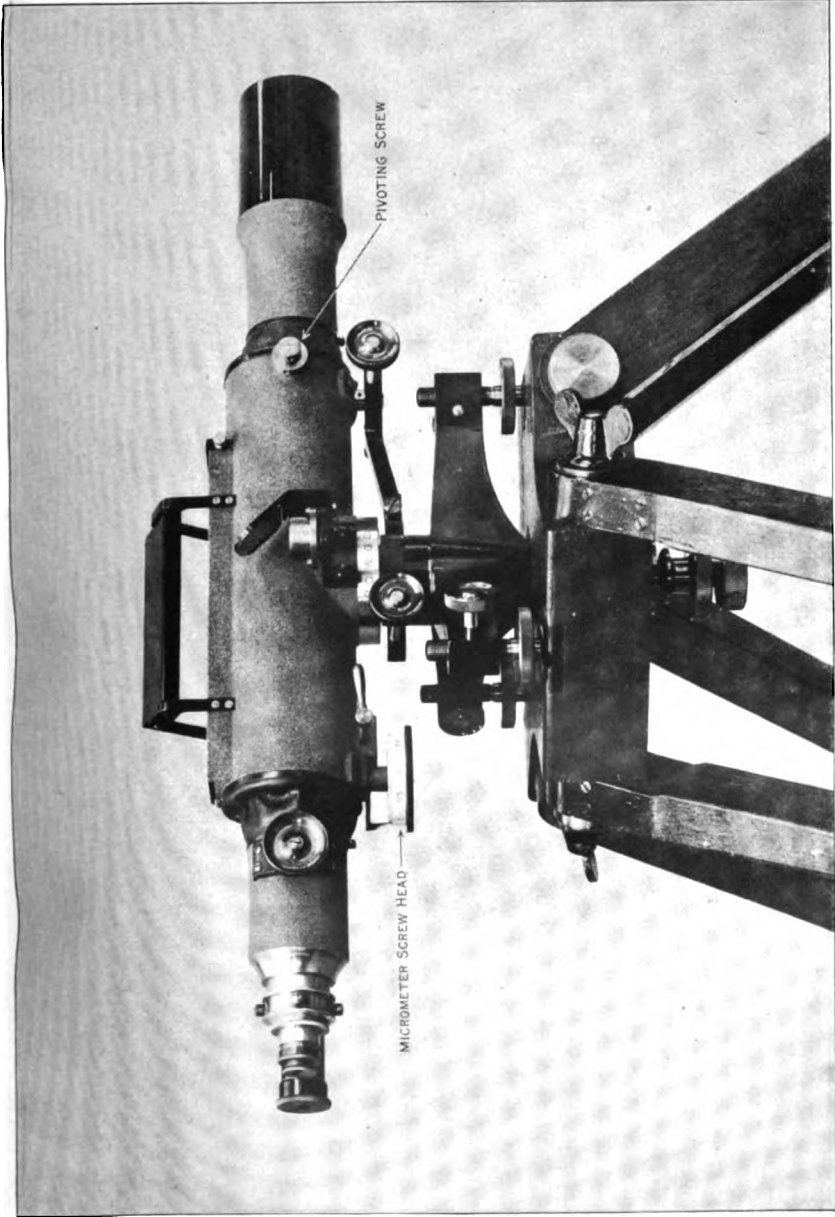
GEODETTIC LEVEL.
